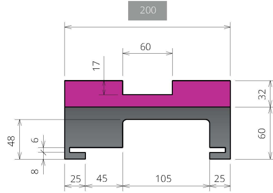
SINGLE TRACK - G00003-a6-T1-BK5-Rm2-P0-L3
