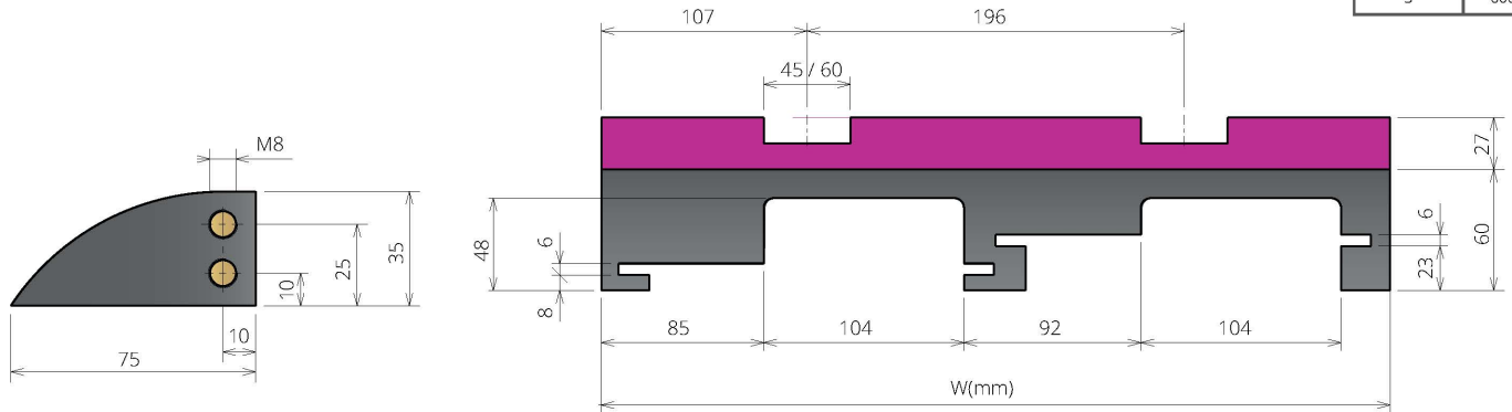
MULTI TRACK - G00003-a6-T2-B6-Rm2-P7-L2
