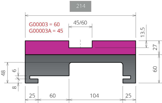
SINGLE TRACK - G00003-a6-T1-B6-Rm2-P0-L1
