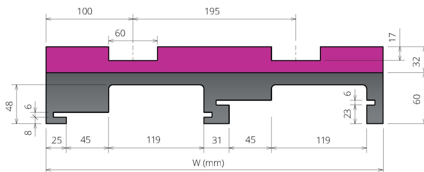
MULTI TRACK - G00003-a6-T2-B5-Rm2-P6-L0
