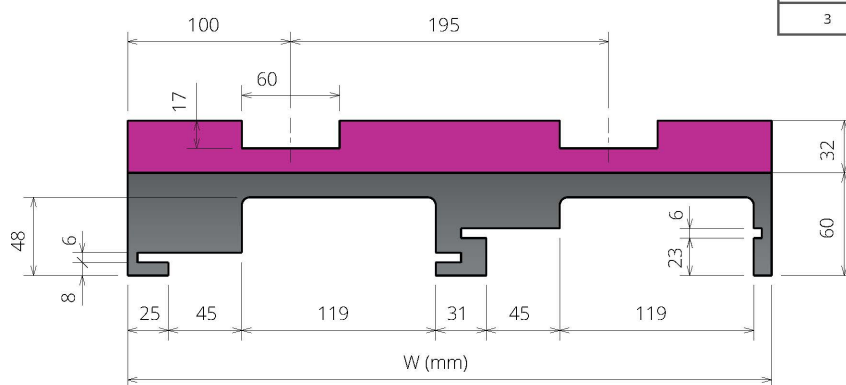
MULTI TRACK - G00003-a6-T2-B5-Rm2-P6-L2
