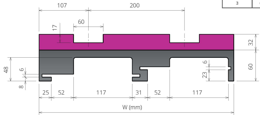
MULTI TRACK - G00003-a6-T2-B6-Rm5-P8-L0
