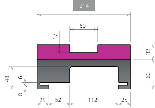
SINGLE TRACK - G00003-a6-T1-B6-Rm5-P0-L0
