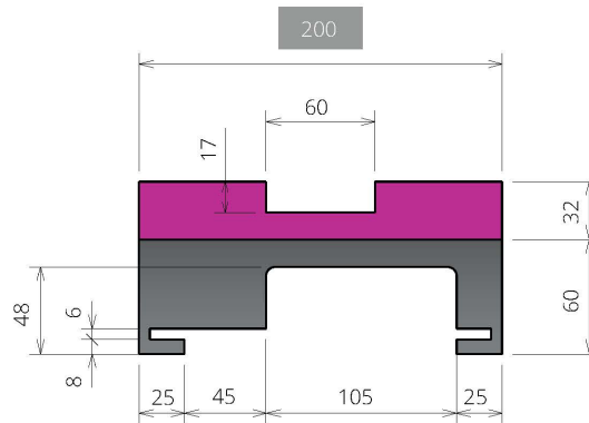
SINGLE TRACK - G00003-a6-T1-B5-Rm2-P0-L1
