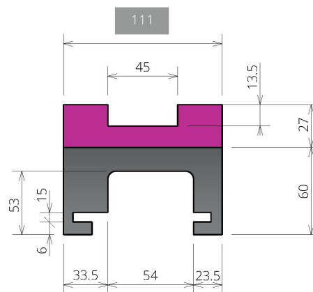
TRACKS W 1 111 2 196 3 281 4 366 5 451 6 536 7 621 8 706
